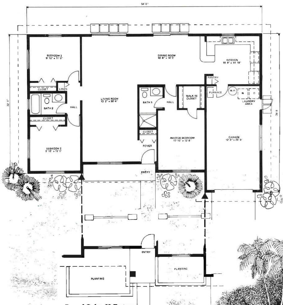
Royal Palm II Entry
